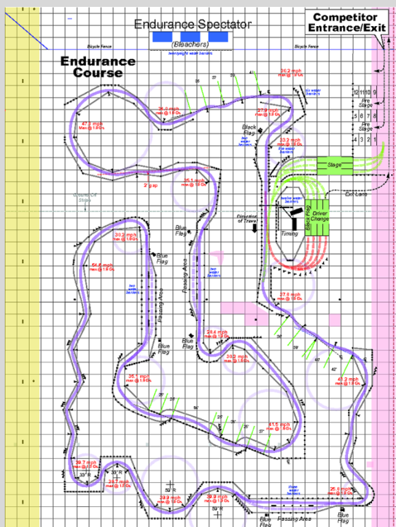
Endurance course for 2015 FSAE Lincoln race
